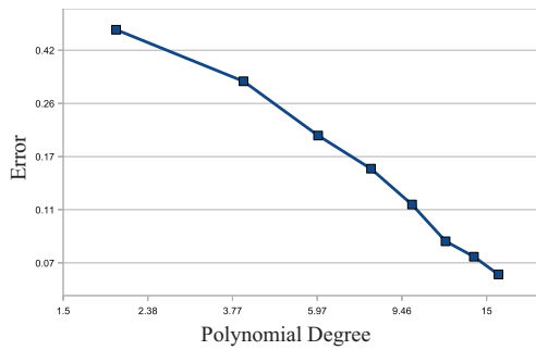
Figure 1: Log-Log plot of accuracy vs. polynomial degree for analysis of a PDE.
